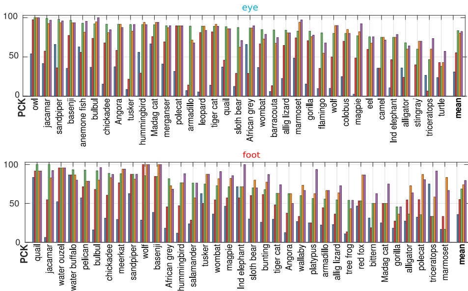
Figure 2: Relative difficulty of part detection and part transfer. Part detection performance for eyes (top) and feet (bottom) for a subset of the target classes, where the detector has been trained using either: ■ the farthest class (in semantic distance), ■ the nearest class, ■ the same class, ■ the source classes, ■ all source and target classes. Classes are sorted by increasing difficulty.
