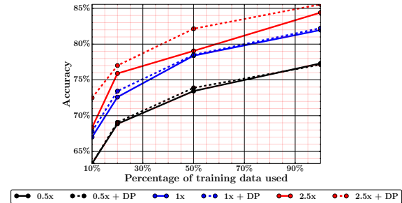
(a) Different pretrained network widths w/ and w/o Dropout
