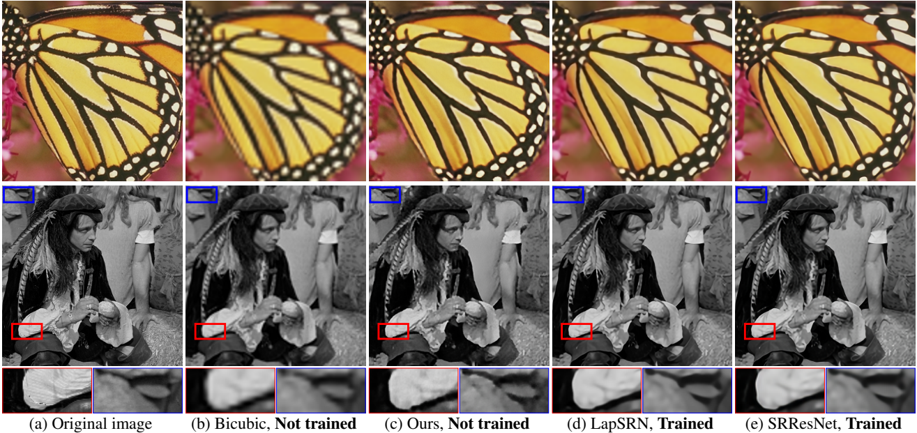
Figure 5: 4x image super-resolution. Similarly to e.g. bicubic upsampling, our method never has access to any data other than a single low-resolution image, and yet it produces much cleaner results with sharp edges close to state-of-the-art super-resolution methods (LapSRN [18], SRResNet [19]) which utilize networks trained from large datasets.
